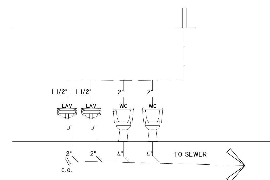
3 PLUMBING RISER DIAGRAM Scale: NTS
