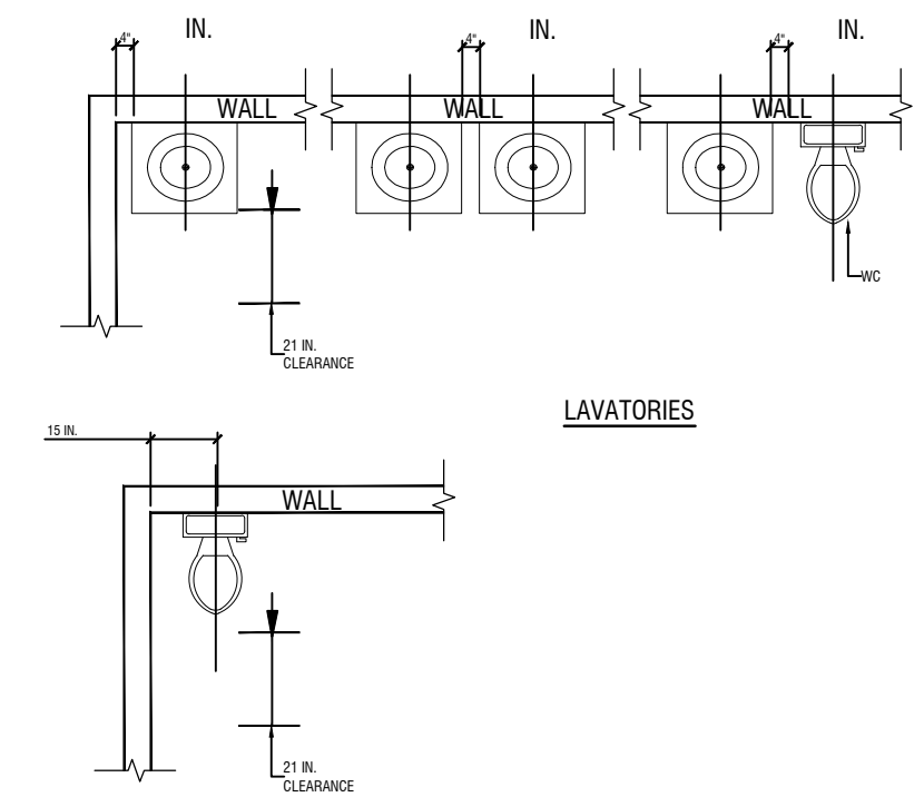
4 BATHROOM FIXTURE CLEARANCE
